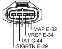
TMAP Manifold Absolute Pressure Temperature Sensor
