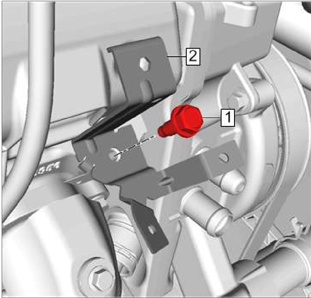
Fig 6: Heater Hose Bracket And Bolt
