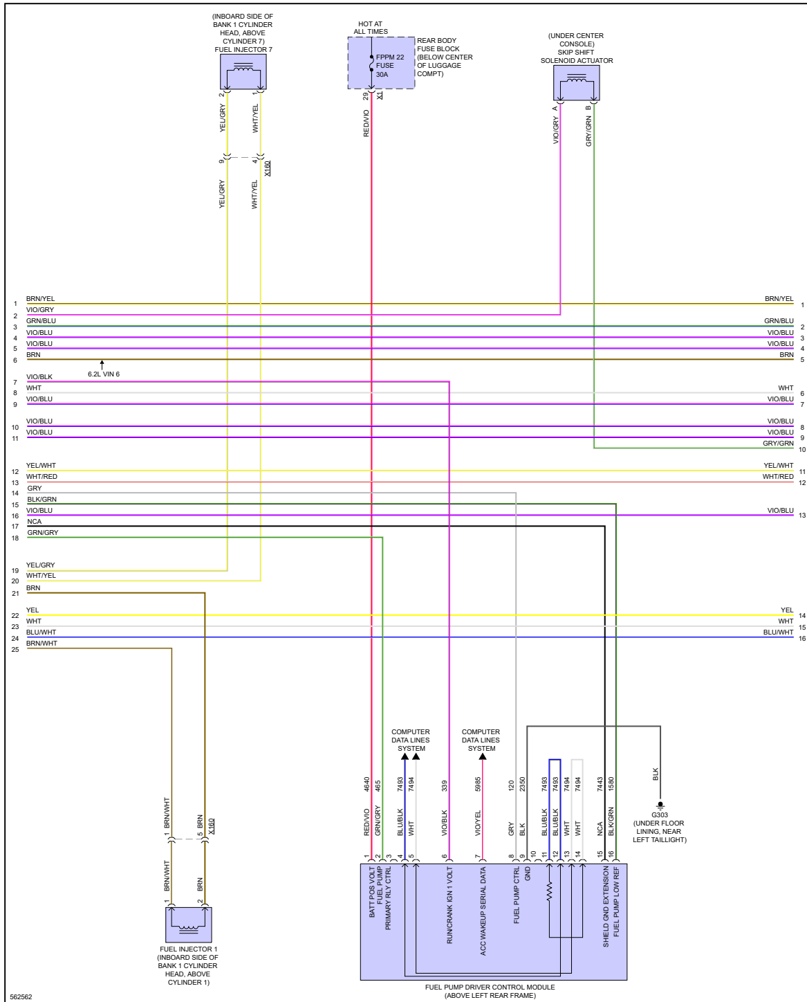
Fig 7: 6.2L VIN 6, Engine Performance Circuit (7 of 9)
