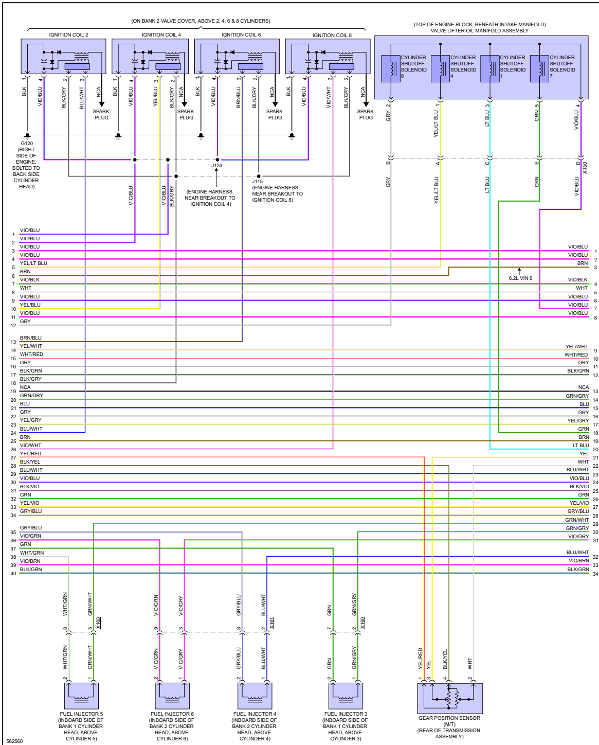
Fig 5: 6.2L VIN 6, Engine Performance Circuit (5 of 9)
