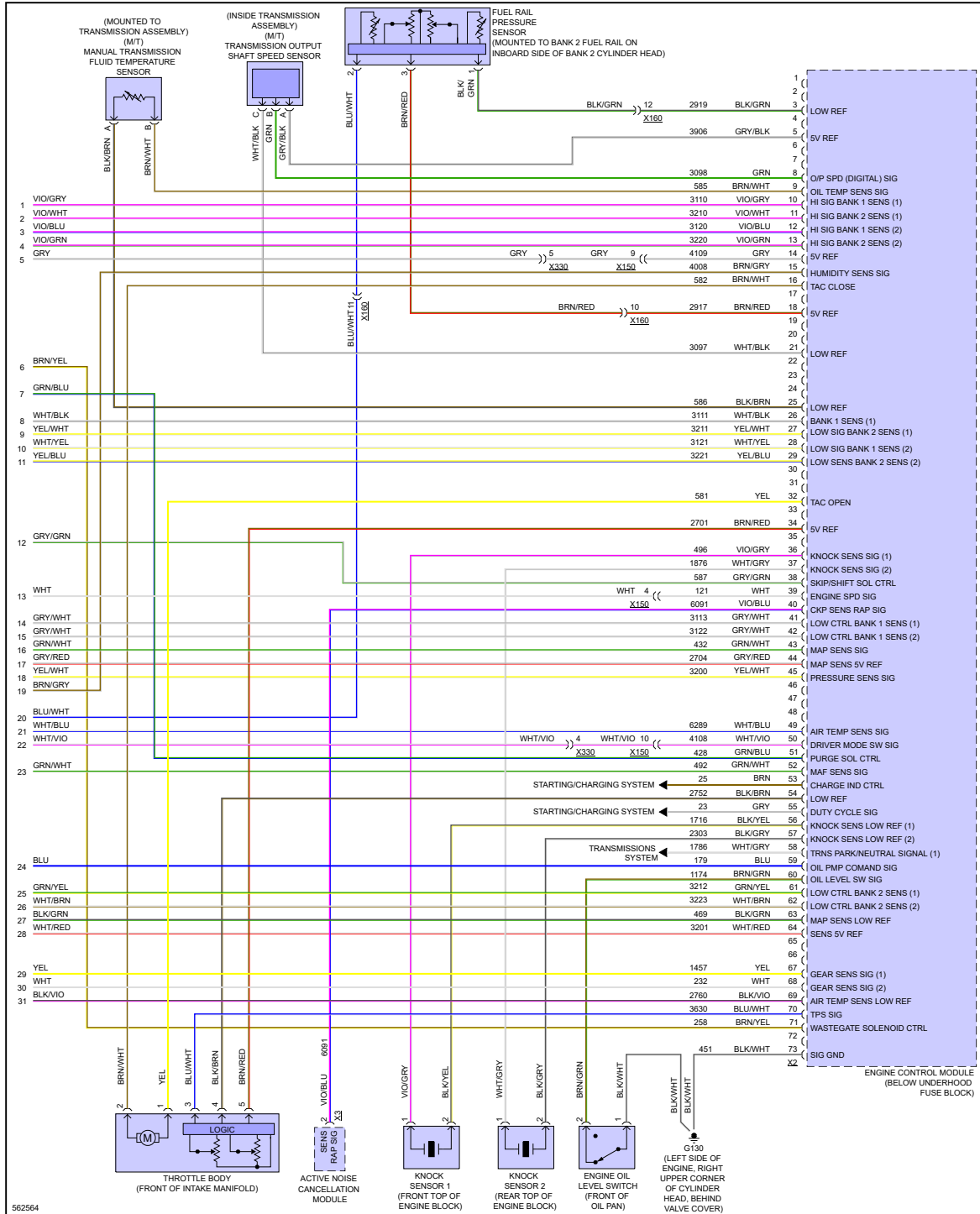
Fig 9: 6.2L VIN 6, Engine Performance Circuit (9 of 9)
