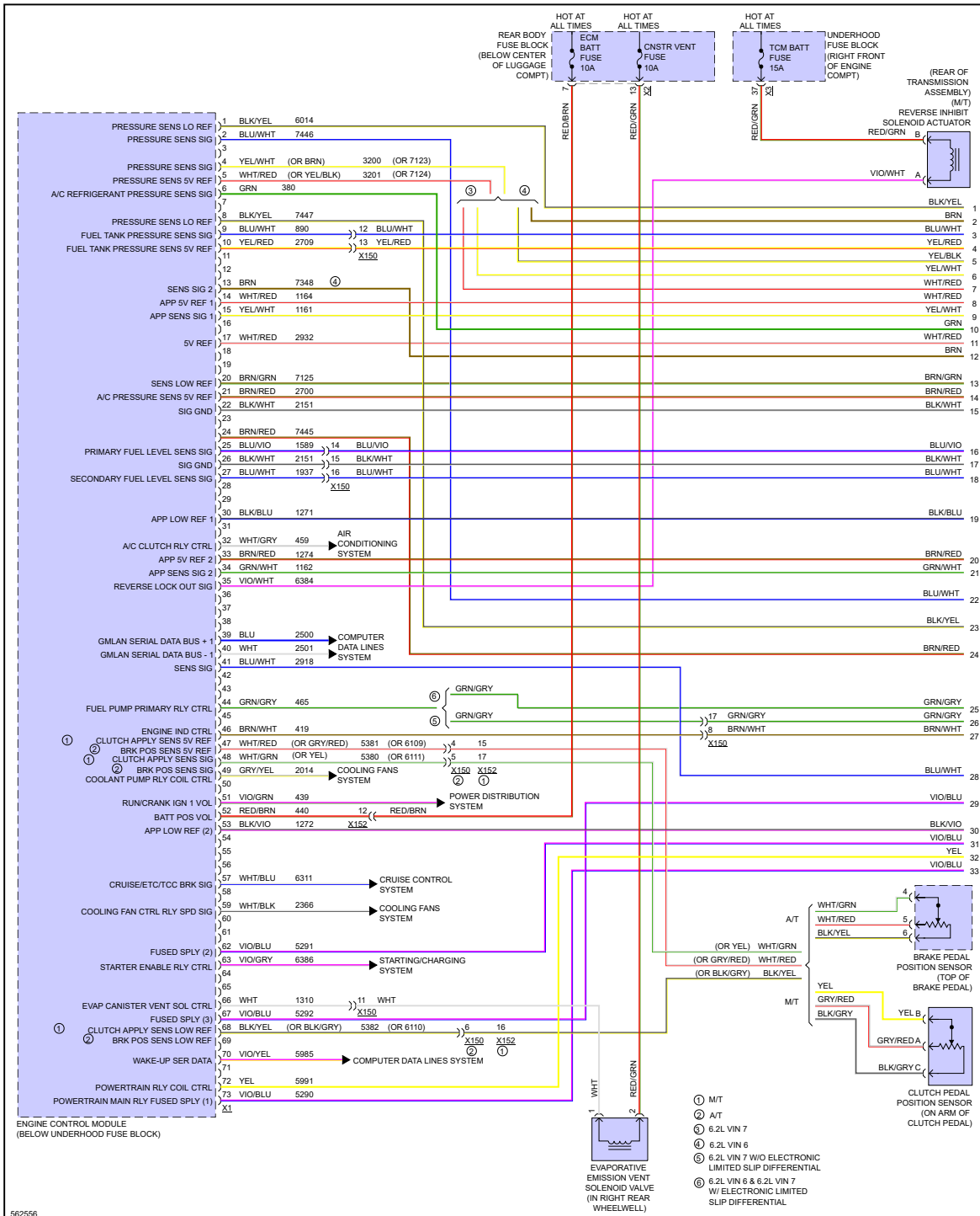
Fig 1: 6.2L VIN 6, Engine Performance Circuit (1 of 9)
