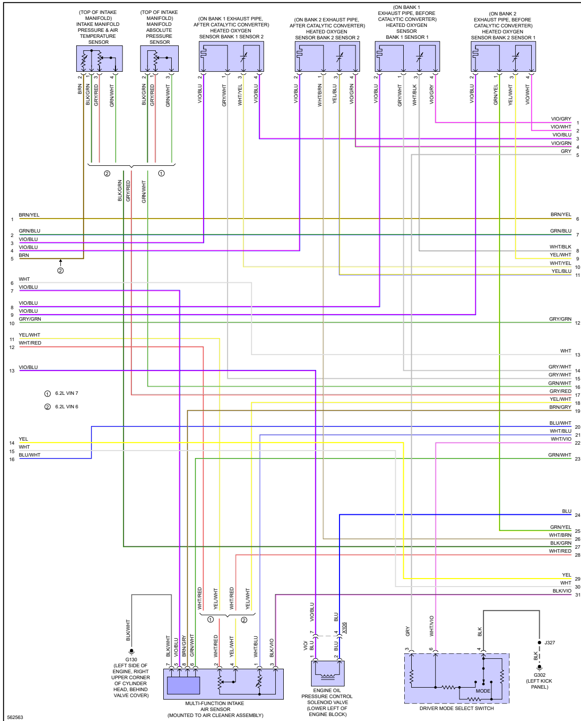
Fig 8: 6.2L VIN 6, Engine Performance Circuit (8 of 9)
