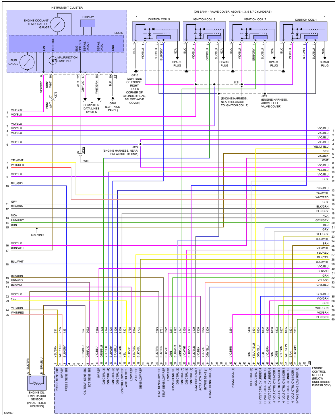
Fig 4: 6.2L VIN 6, Engine Performance Circuit (4 of 9)
