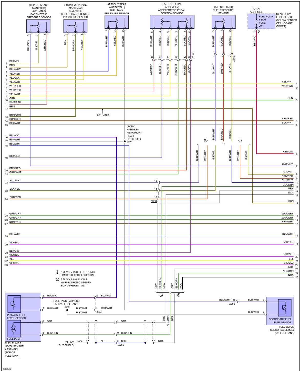
Fig 2: 6.2L VIN 6, Engine Performance Circuit (2 of 9)
