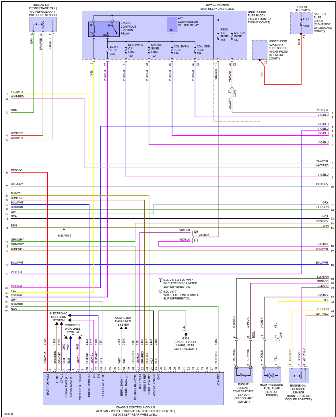
Fig 3: 6.2L VIN 6, Engine Performance Circuit (3 of 9)
