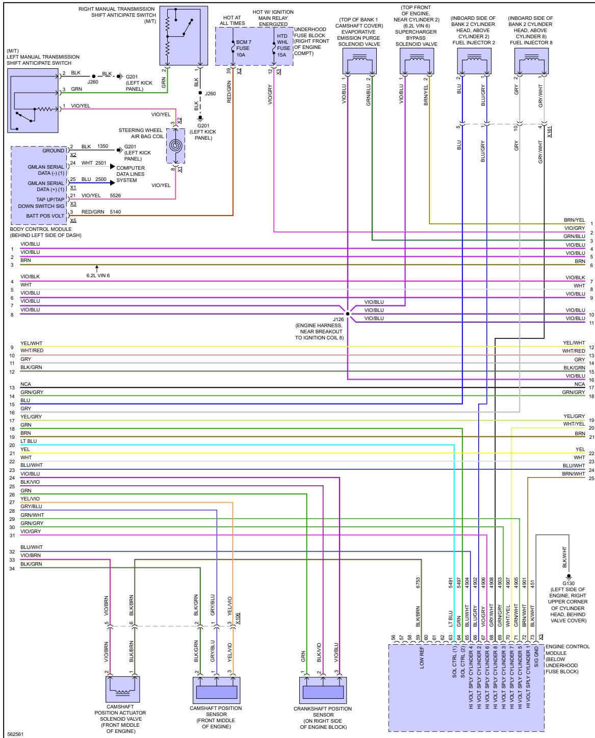
Fig 6: 6.2L VIN 6, Engine Performance Circuit (6 of 9)
