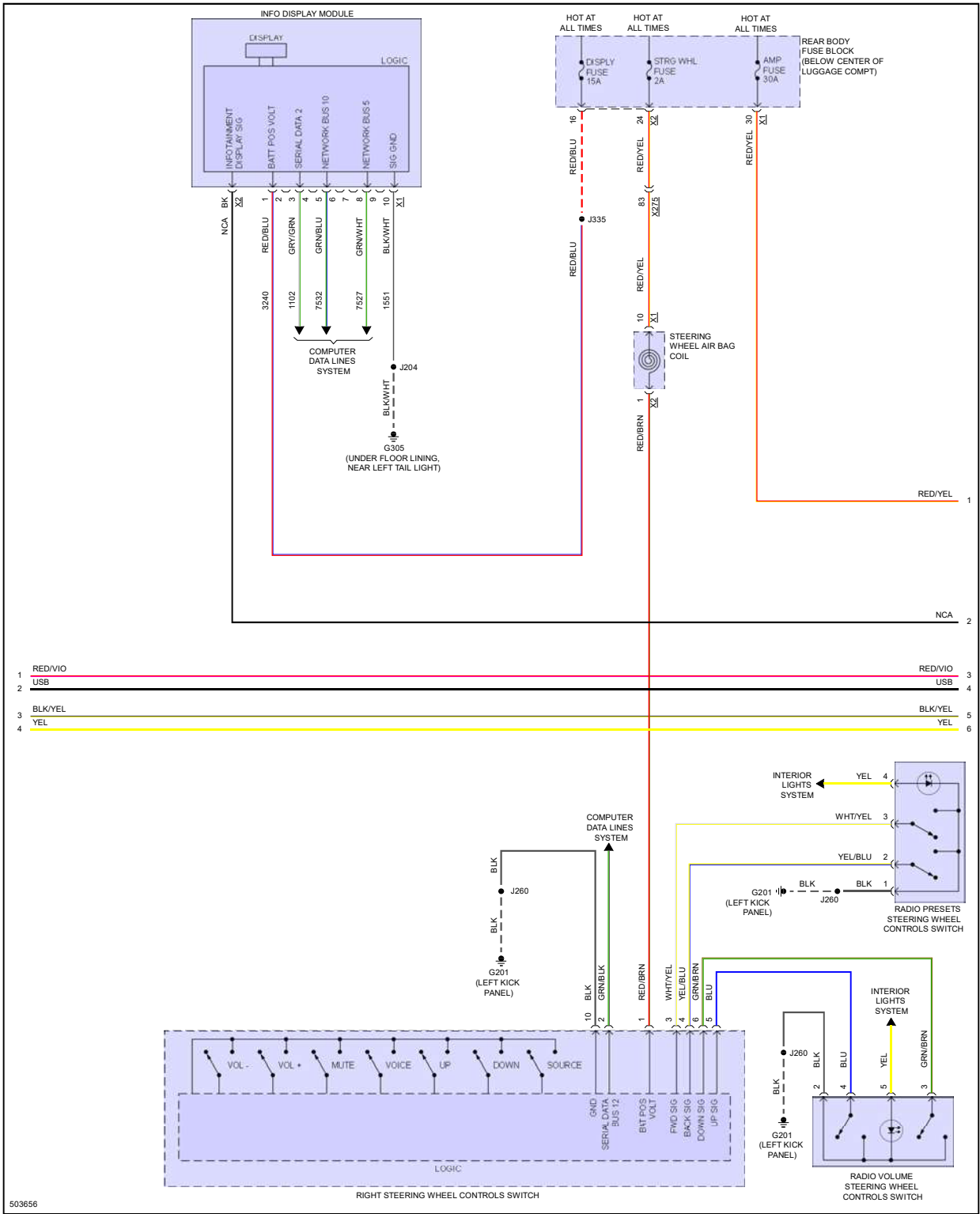
Fig 18: Radio Circuit, W/ Navigation (2 of 5)
