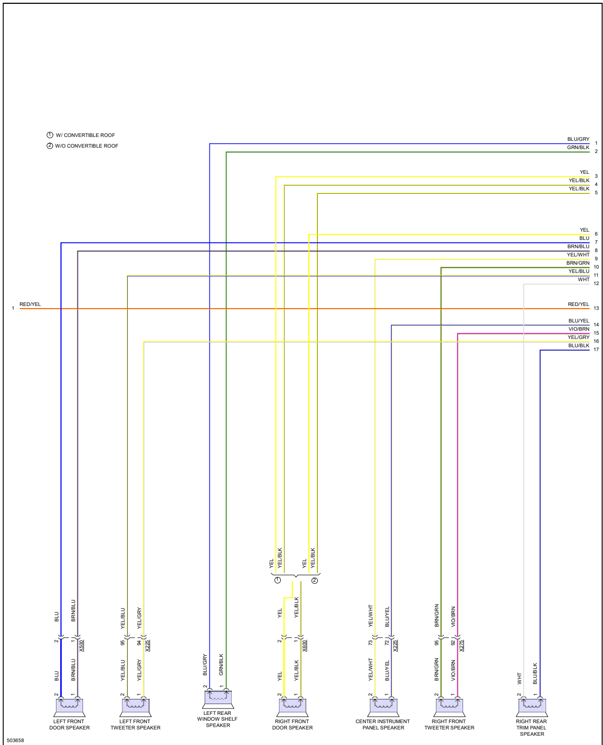
Fig 20: Radio Circuit, W/ Navigation (4 of 5)
