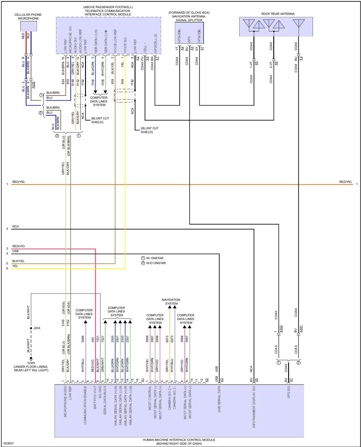
Fig 19: Radio Circuit, W/ Navigation (3 of 5)
