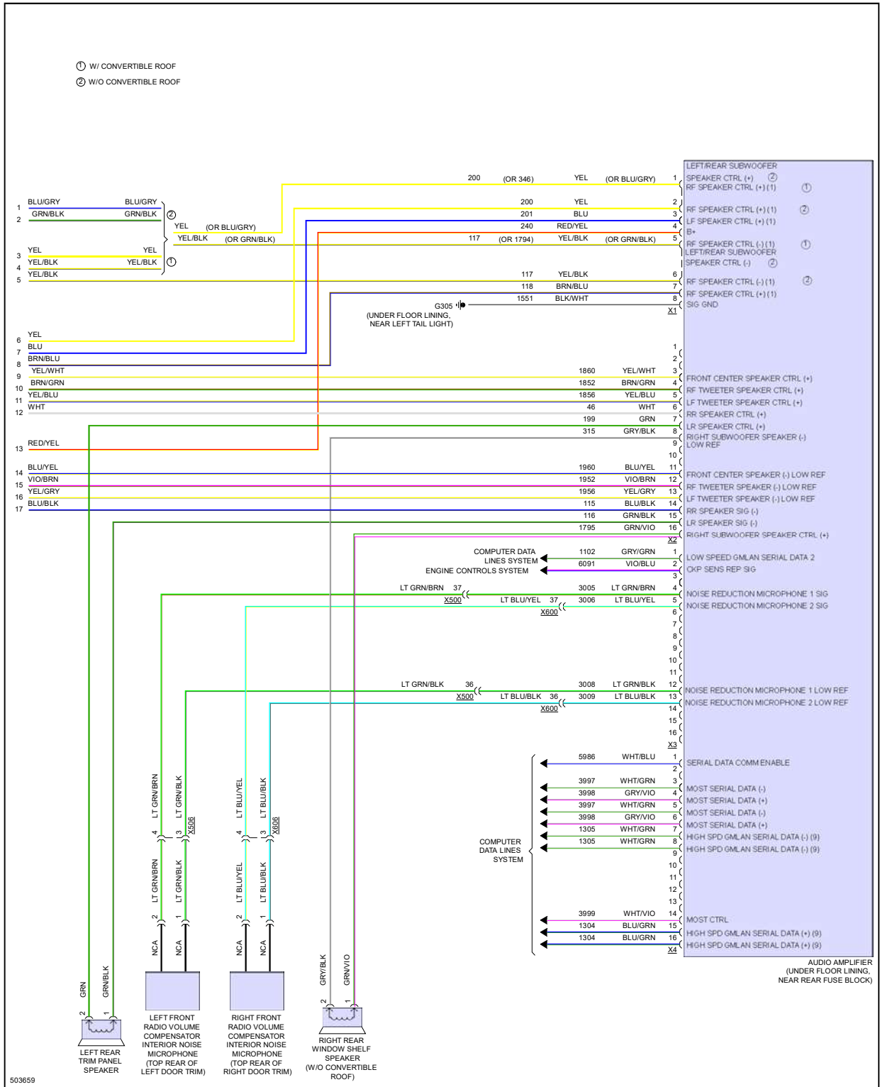
Fig 21: Radio Circuit, W/ Navigation (5 of 5)
